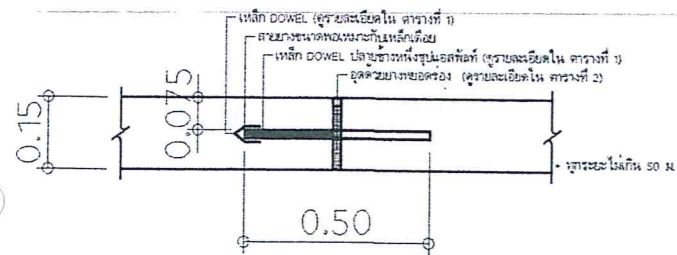
EXPANSION JOINT
