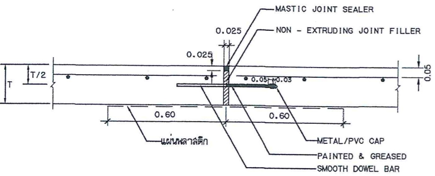
EXPANSION JOINT
