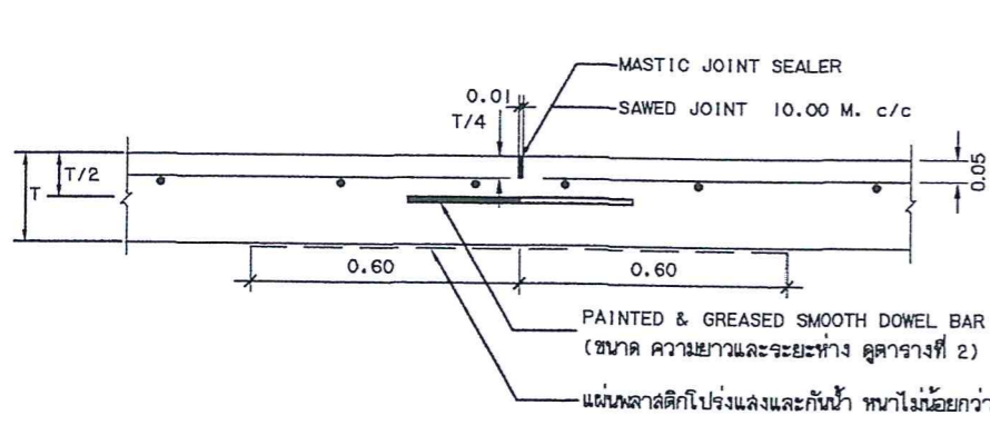
CONTRACTION JOINT
