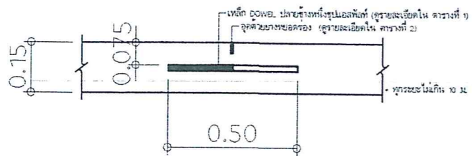
CONTRACTION JOINT
